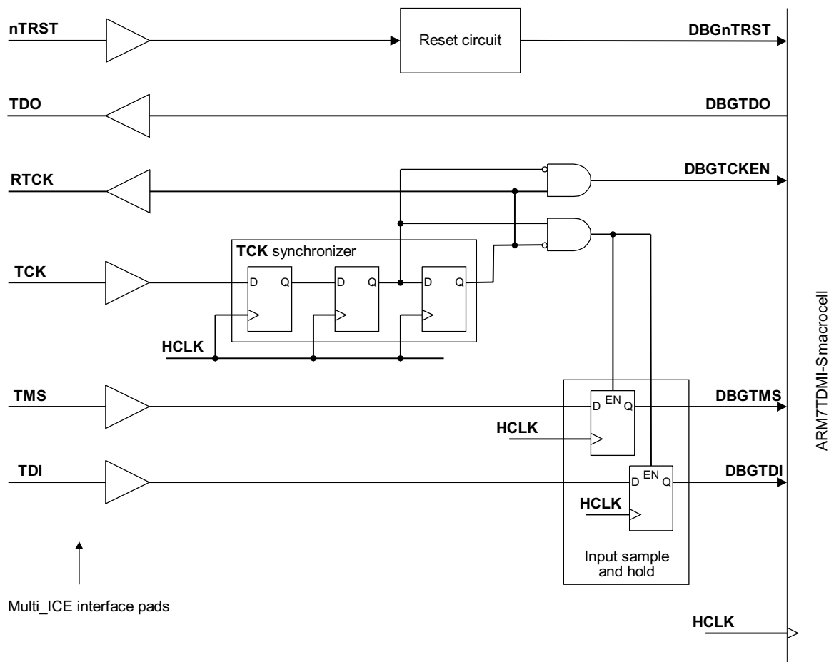
Figure 9-4 Clock synchronization
